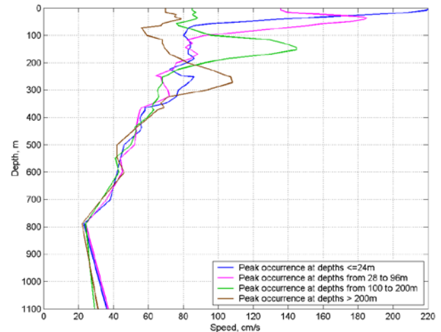
New Gendalo Extreme Current Summary: Maximum Current Speed Profiles for 100-Year Return Periods Characterized by Current Intensification in Different Layers
